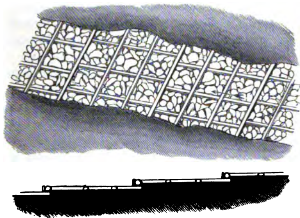
Fig. 251.—Fixing the bed of a stream.
